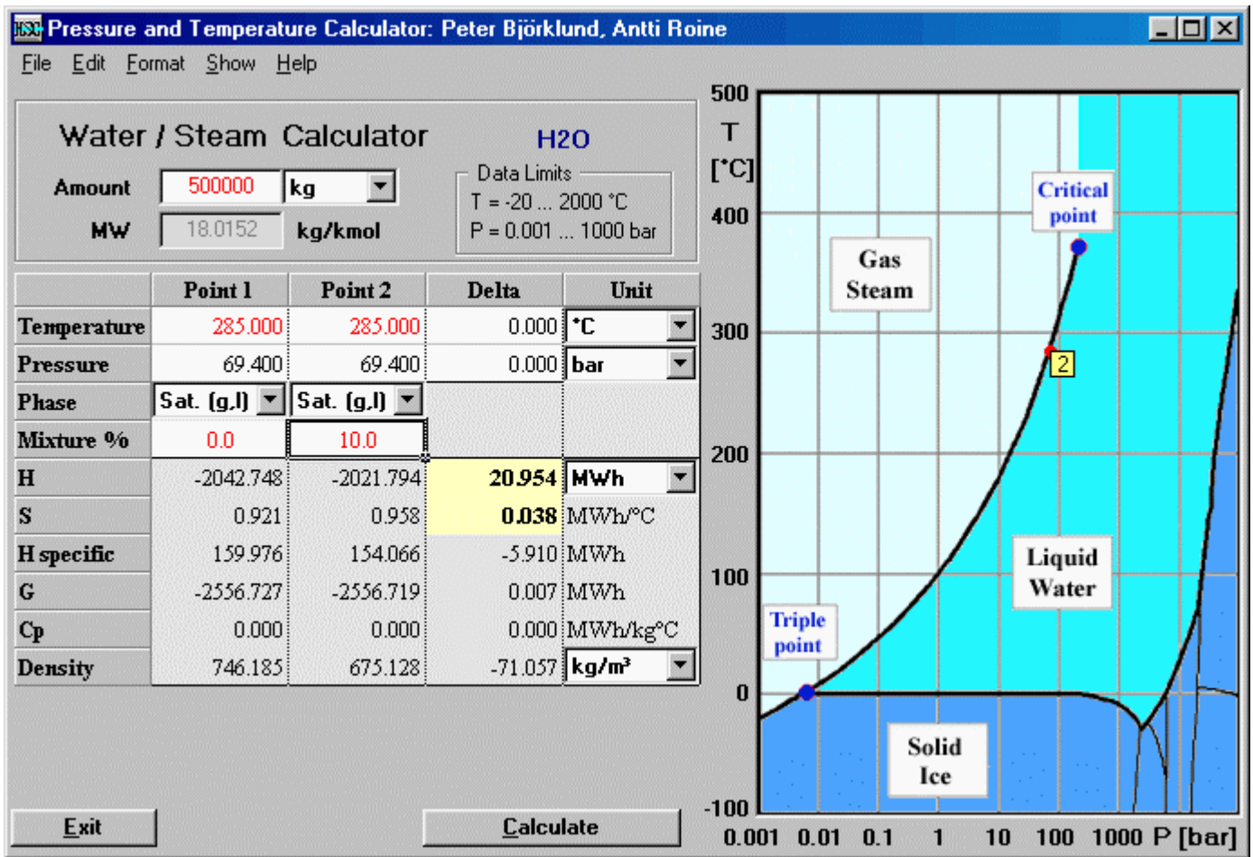
Figure 3: Evaporation process.
